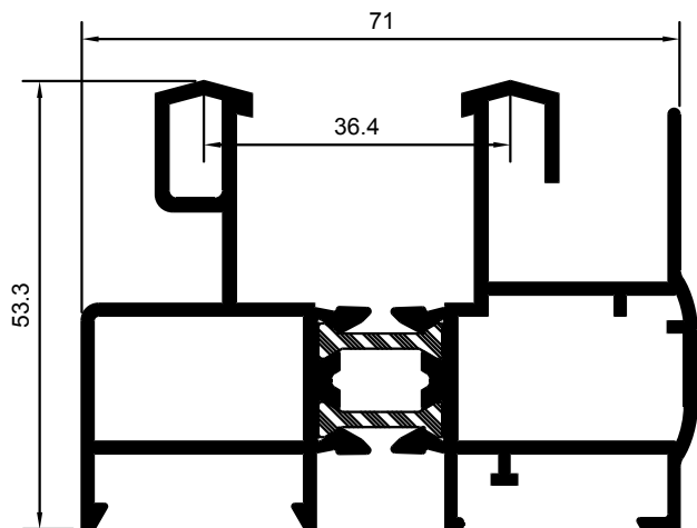
MARCO PERIMETRAL
