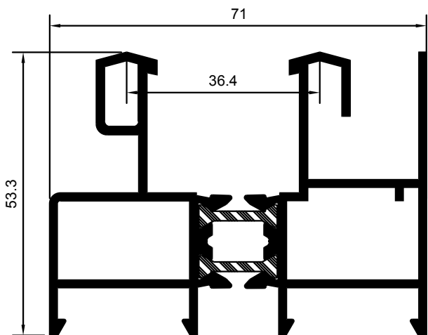
MARCO PERIMETRAL
