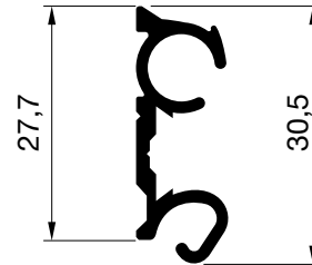
E-2046 Peso: 245 gr/m. P. Total: 124 mm.
