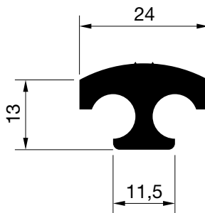
E-3604 Peso: 537 gr/m. P. Total: 92 mm.
