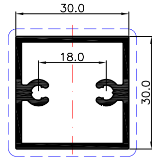
P01626 0.604 Kg/m 0.120 m 2 /m
