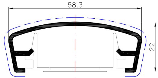
P03332 0.476 Kg/m 0.227 m 2 /m
