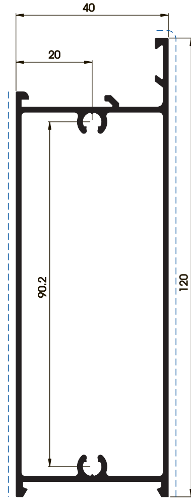
P01945 1,562 kg/m 0,370 m 2 /m
