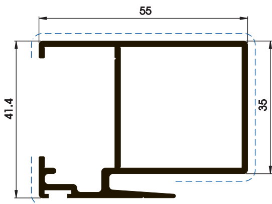
P03270 0,886 kg/m 0,300 m 2 /m
