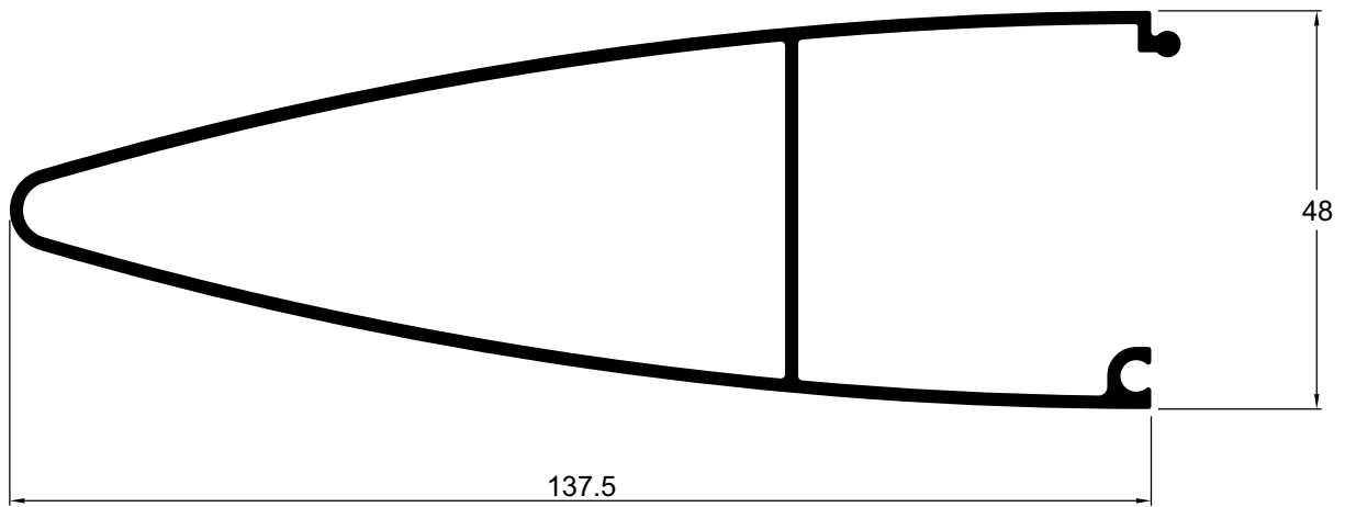
DC008 1,569 kg/m Brise
