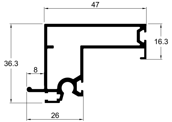
VL117 0,774 kg/m Travessa inferior/superior
