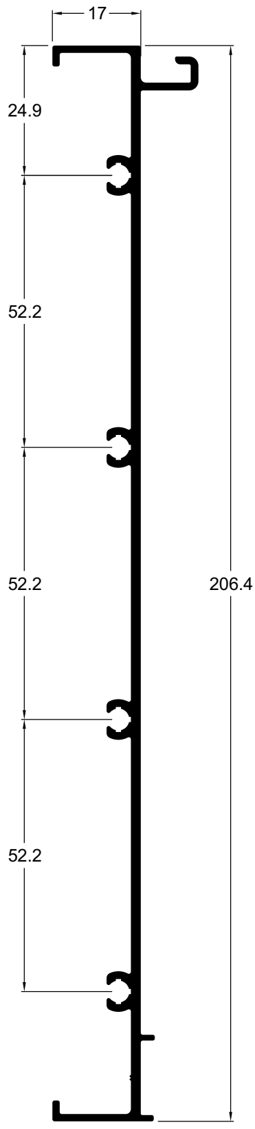
GN083 1,490 kg/m Marco trav. int. 3 planos integrada
