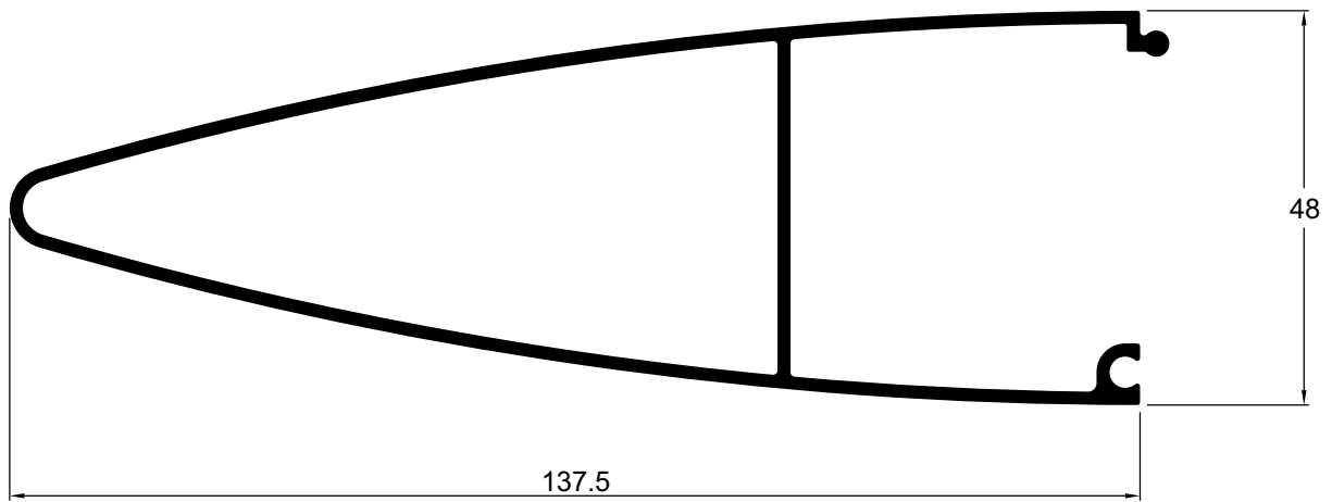
DC008 1,505 kg/m Brise
