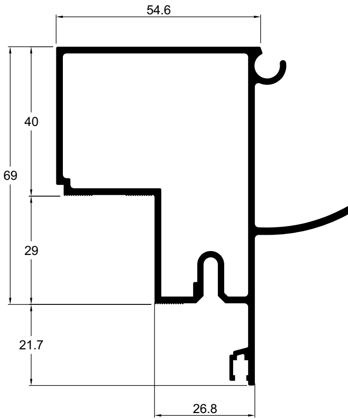
VL035 1,577 kg/m
